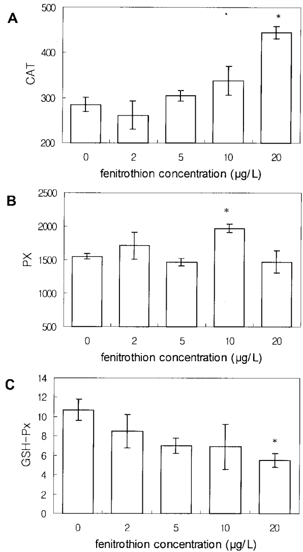
Fig. 2. Effects of fenitrothion exposure on catalase (CAT; A), peroxidase (Px; B), glutathione peroxidase (GSH-Px; C) activities (mean \pm s.e.; n = 5 ) measured in 4 th instar larvae of Ch. riparius . Enzymatic activities are expressed as unit-mg -1 protein. *: significantly different from control, p < 0.05 .
